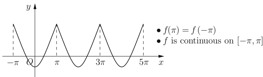
Fig. 10.5. Periodic extension of f from [-\pi, \pi] with f(\pi) = f(-\pi) to \mathbb{R} .
