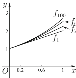
Fig. 9.29. f_n(x) = (1 + x/n)^n on [0, 1] .
