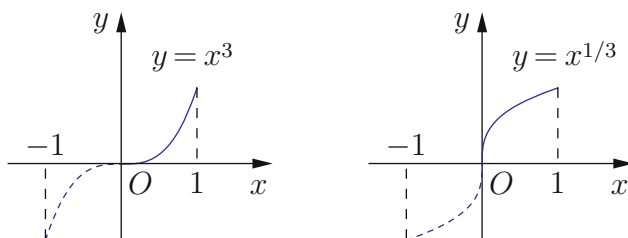
Fig. 4.4. Graphs of y = x^3 and y = x^{1/3} on [-1, 1] .
