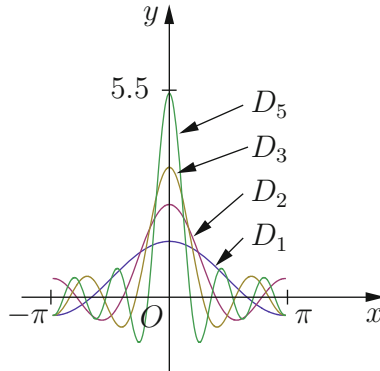
Fig. 10.21. The graph of D_n(t) = \frac{1}{2} + \sum_{k=1}^n \cos(kt) for certain values of n .
