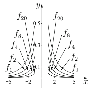
Fig. 9.6. f_n(x) = 1/(1+nx^2) on [-5, -1] \cup [1, 5] .
