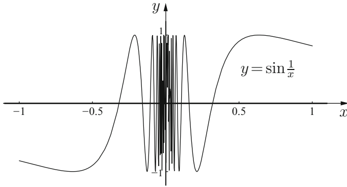
Fig. 3.1. Graph of f(x) = \sin(1/x) on [-1, 1] .
