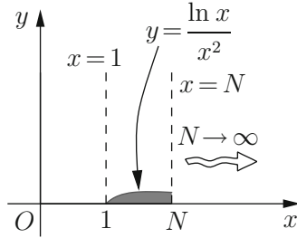
Fig. 7.6. Area under y = (\ln x)/x^2 on [1, N] for large N .
