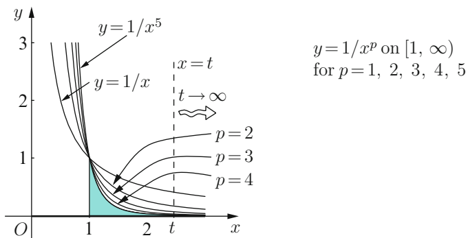
Fig. 7.5. Convergence of the integral \int_1^\infty (1/x^p) dx , for p \in [1, \infty) .
