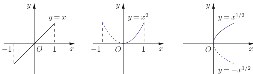
Fig. 4.3. Graphs of y = x , y = x^2 on [-1, 1] , and y = x^{1/2} on [0, 1] .
