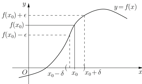
Fig. 3.4. Depiction of the continuity of f at x_0 .
