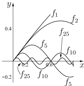
Fig. 9.37. Graph of f_n(x) = (\sin nx)/n .
