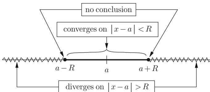
Fig. 8.4. Finite radius R of convergence of \sum_{k \geq 1} a_k(x-a)^k .
