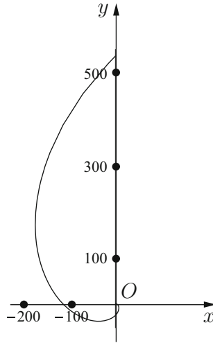
Fig. 7.30. The curve x = e^\theta \sin \theta , y = e^\theta \cos \theta for 0 \leq \theta \leq 2\pi .
