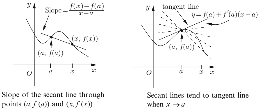
Fig. 3.10. Depiction of differentiability of f at a .
