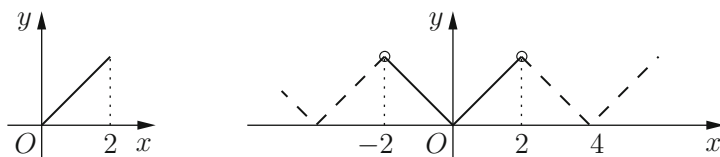
Fig. 10.16. Even extension of f(x) = x for 0 < x < 2 , period 4.
