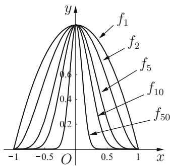
Fig. 9.20. f_n(x) = (1 - x^2)^n on [-1, 1] .
