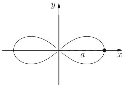
Fig. 7.33. Graph of r^2 = a^2 \cos 2\theta .
