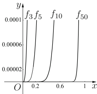
Fig. 9.19. f'_n(x) = x^{n-1} on (-1, 1) .
