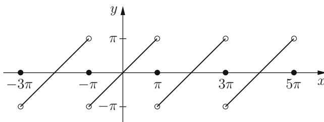
Fig. 10.12. Graphs of f(x) = f(x + 2\pi) , f(x) = x on (-\pi, \pi) with f(\pi) = 0 = f(-\pi) .
